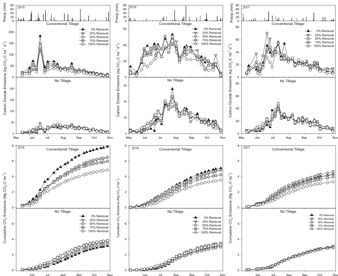
FIGURE 1 Episodic (upper graphs) and cumulative (lower graphs) \text{CO}_2 emissions under no-tillage and conventional tillage at five stover removal rates (0, 25, 50, 75, and 100%) in the 2015, 2016, and 2017 growing seasons. Note the different y-axis scales for the \text{CO}_2 emission data. The upper bar graph is the daily precipitation for the 2015, 2016, and 2017 growing seasons
